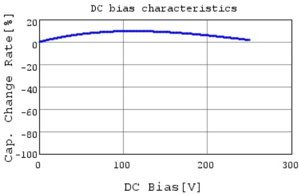
DE2E3KY152MN2AM01F C-DC bias capchange, 20.0
