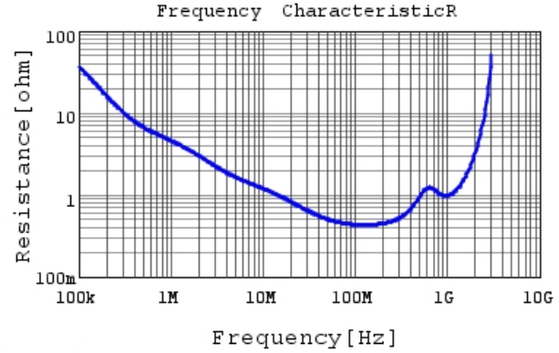
DE2E3KY152MN2AM01F R DCOV, 20degC
