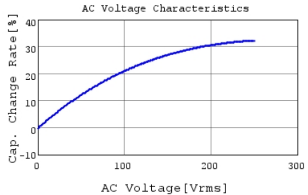
DE2E3KY152MN2AM01F C-AC Voltage capchange, I
