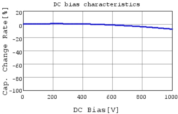
DE1B3RA221KN4AP01F C-DC bias capchange, 20.0
