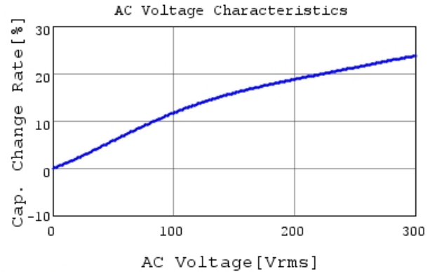
DE1B3RA221KN4AP01F C-AC Voltage capchange, I
