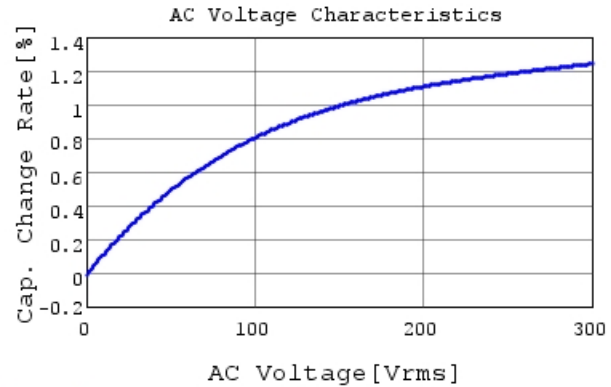
DE11XRA330KJ4BP01F C-AC Voltage capchange, I
