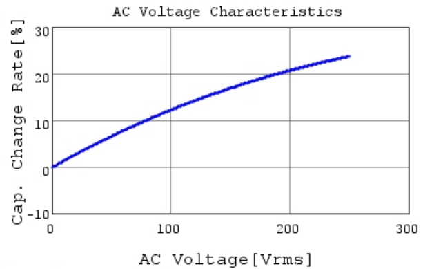
DE1E3KX332MJ4BN01F C-AC Voltage capchange, I
