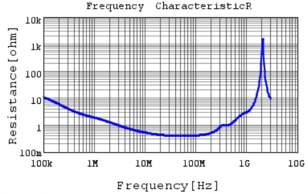
DE1E3KX332MJ4BN01F R DCOV, 20degC
