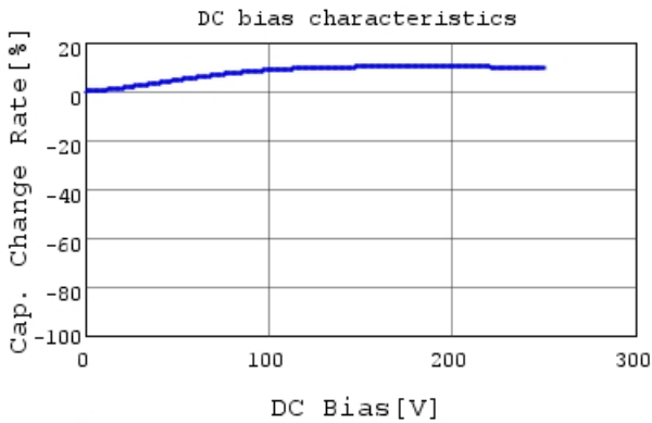
DE1E3KX332MJ4BN01F C-DC bias capchange, 20.0
