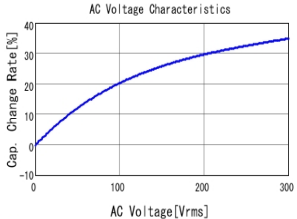
■ DE2B3KY221KA3BU02F C-AC Voltage capchange, DC0V, 20.0
