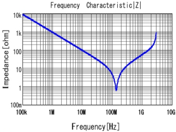
■ DE2B3KY221KA3BU02F |Z| DC0V, 20degC
