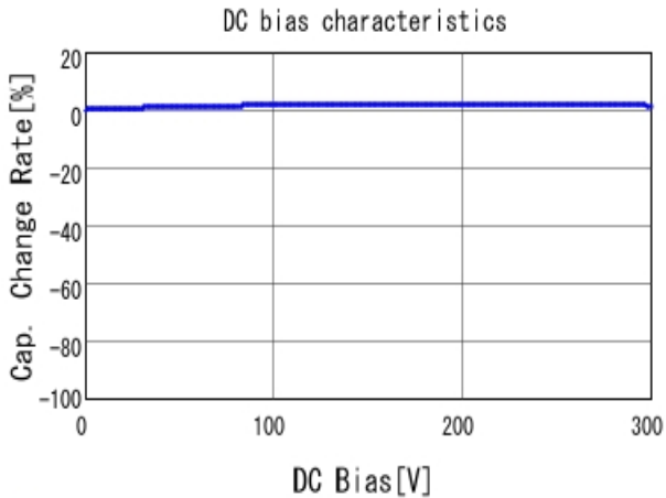
■ DE2B3KY221KA3BU02F C-DC bias capchange, 20.0degC, AC1
