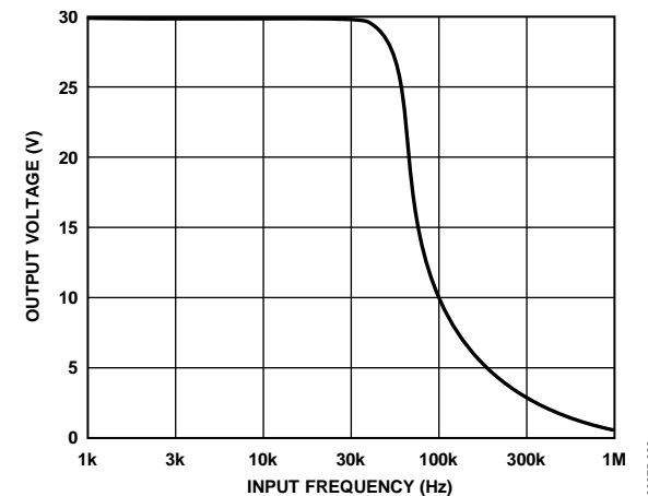
Figure 23. Large Signal Frequency Response
