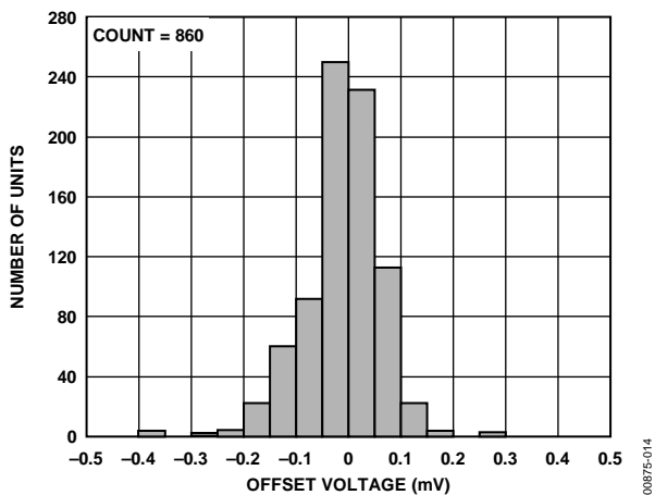
Figure 14. Input Offset Distribution, V_S = 5\text{V}, 0\text{V}
