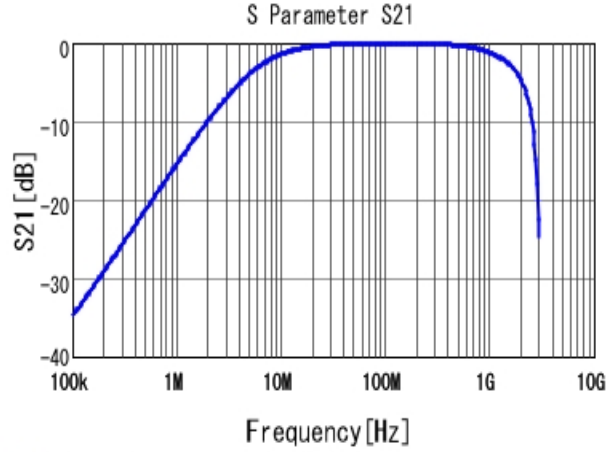
■ DE2B3KY331KN3AM02F S21 DCOV, 20degC
