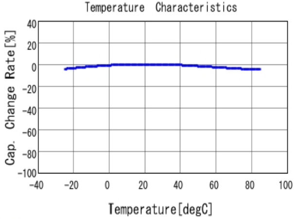
■ DE2B3KY331KN3AM02F C-Temp. capchange, DCOV, AC1Vrms
