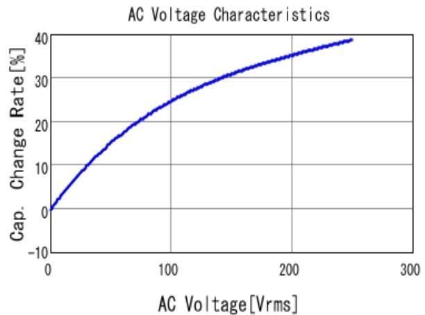
■ DE2B3KY331KN3AM02F C-AC Voltage capchange, DCOV, 20.0
