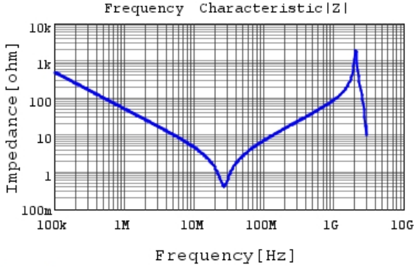
DE1E3KX332MB4BP01F |Z| DC0V, 20degC
