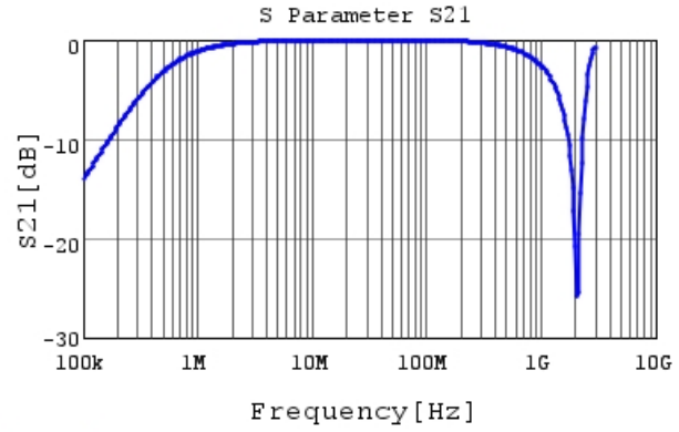
DE1E3KX332MB4BP01F S21 DCOV, 20degC
