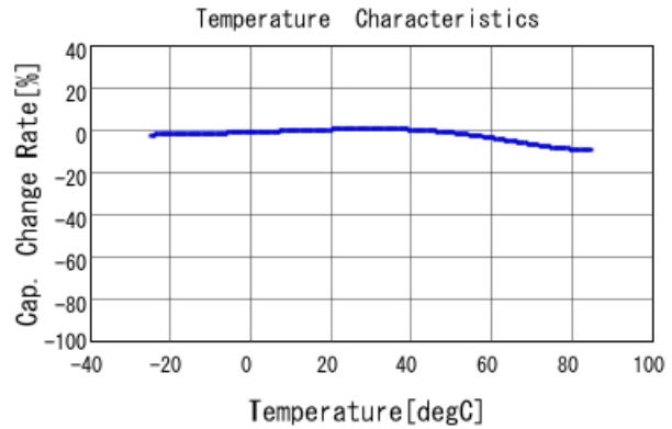
DE2B3SA221KA2BT01F C-Temp. capchange, DCOV, AC1Vrr
