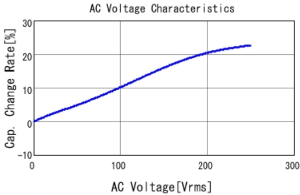
DE2B3SA221KA2BT01F C-AC Voltage capchange, DCOV, 2
