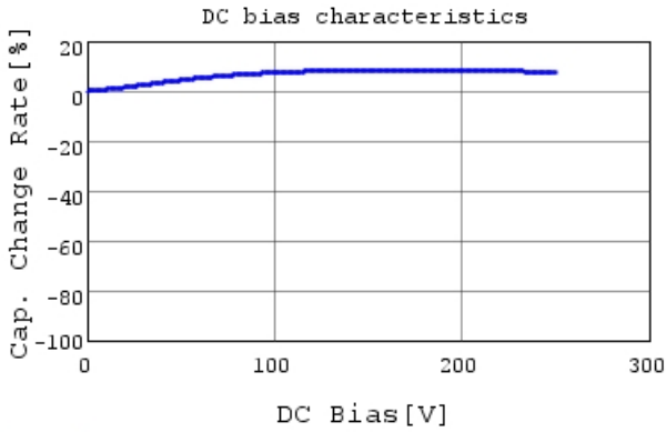
DE1E3KX222MB4BN01F C-DC bias capchange, 20.0
