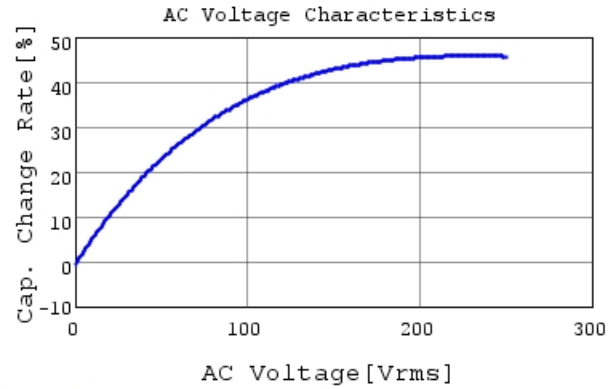
DE1E3KX222MB4BN01F C-AC Voltage capchange, I
