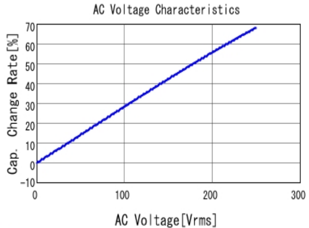
■ DE2B3KY471KB3BM02F C-AC Voltage capchange, DCOV, 20.0
