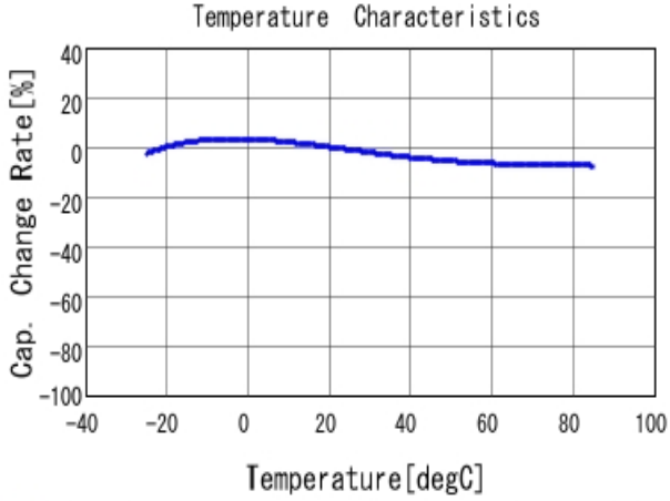
■ DE2B3KY471KB3BM02F C-Temp. capchange, DCOV, AC1Vrms
