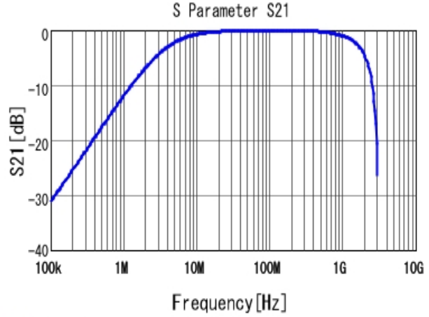
■ DE2B3KY471KB3BM02F S21 DCOV, 20degC
