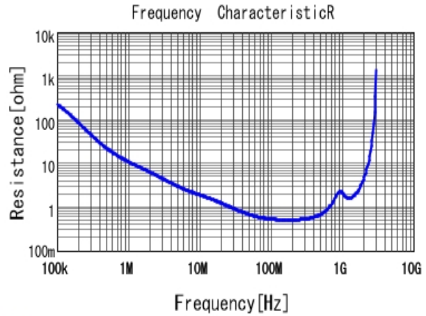
■ DE2B3KY471KB3BM02F R DCOV, 20degC
