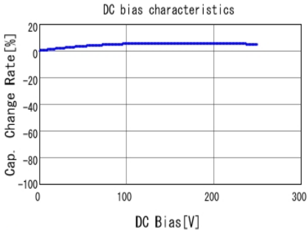
■ DE2B3KY471KB3BM02F C-DC bias capchange, 20.0degC, AC1
