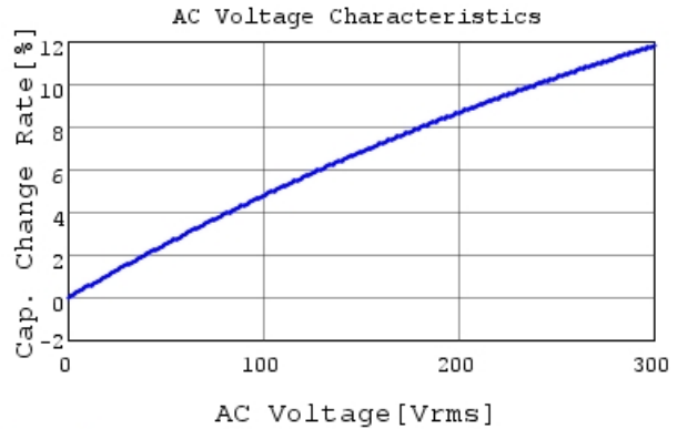
DE1B3KX101KB4BP01F C-AC Voltage capchange, I
