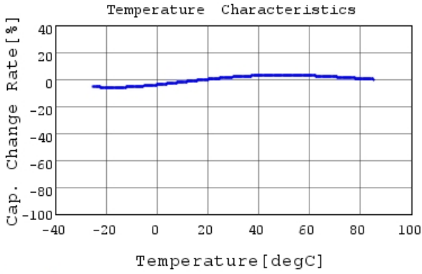
DE1B3KX101KB4BP01F C-Temp. capchange, DCOV,
