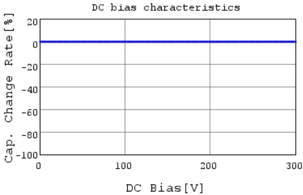
DE1B3KX101KB4BP01F C-DC bias capchange, 20.0
