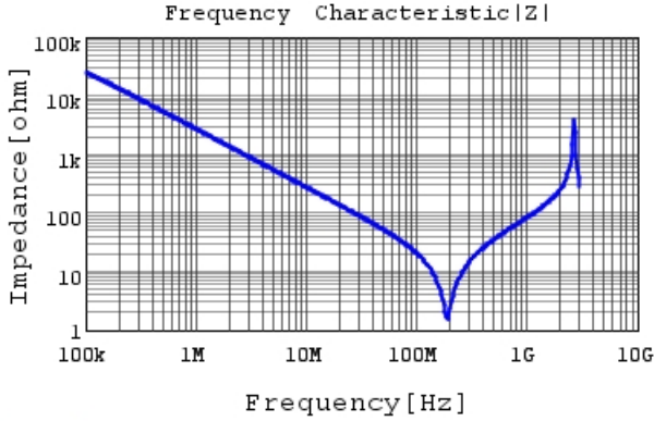
DE1B3KX101KB4BP01F |Z| DC0V, 20degC
