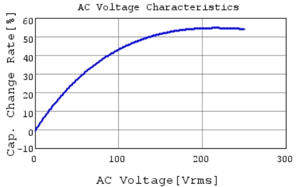
DE2E3KY222MB3BM02F C-AC Voltage capchange, I
