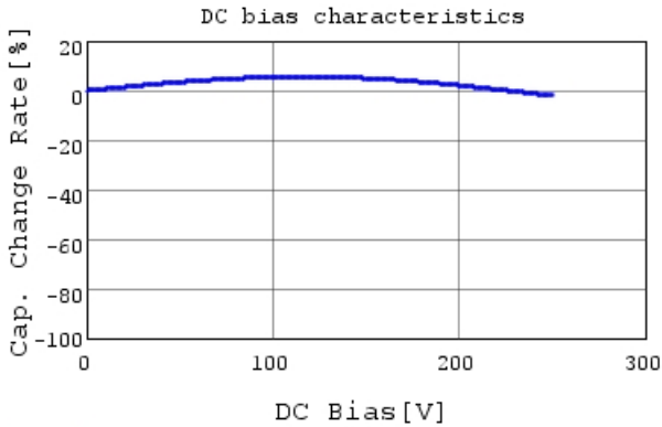
DE2E3KY222MB3BM02F C-DC bias capchange, 20.0
