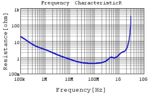
DE2E3KY222MB3BM02F R DC0V, 20degC
