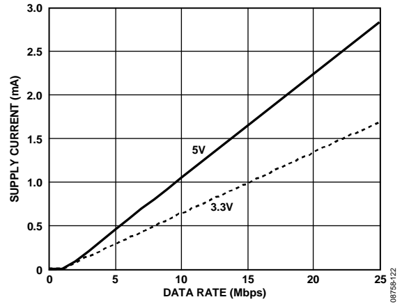
Figure 22. Typical I_{ISO(ID)} Dynamic Supply Current per Output (15 pF Output Load)
