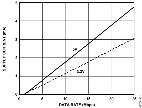
Figure 21. Typical I_{ISO(ID)} Dynamic Supply Current per Input
