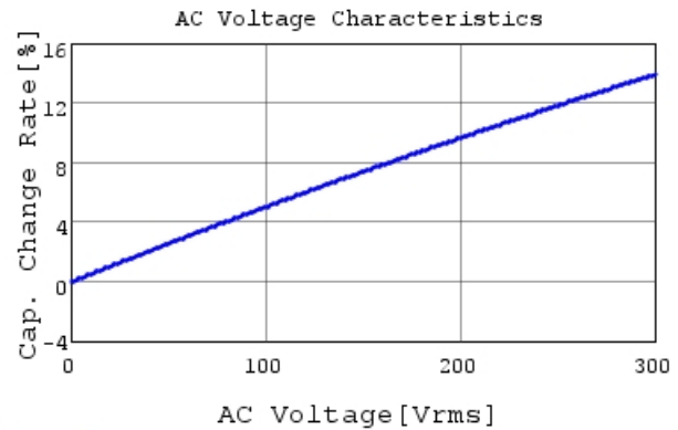
DE1B3KX331KN4AP01F C-AC Voltage capchange, I
