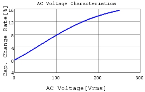
DE1B3RA101KJ4BN01F C-AC Voltage capchange, I
