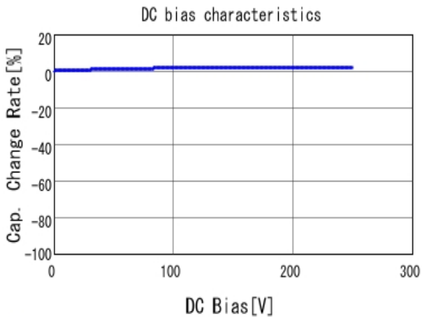
■ DE2B3KY221KB2BM01F C-DC bias capchange, 20.0degC, AC1
