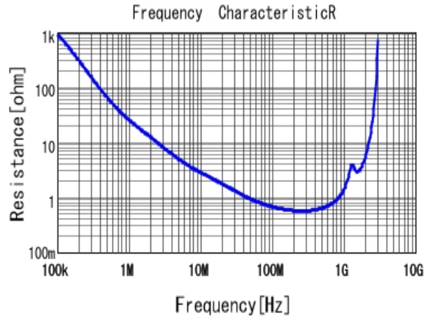
■ DE2B3KY221KB2BM01F R DCOV, 20degC
