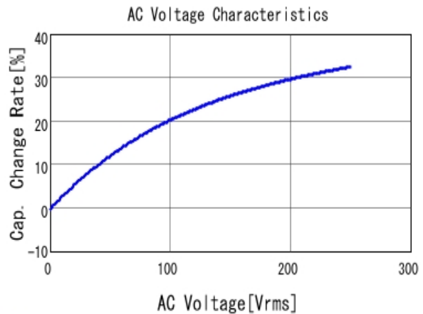
■ DE2B3KY221KB2BM01F C-AC Voltage capchange, DCOV, 20.0
