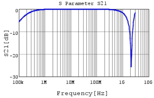
DE2F3KY103MA3BU02F S21 DCOV, 20degC
