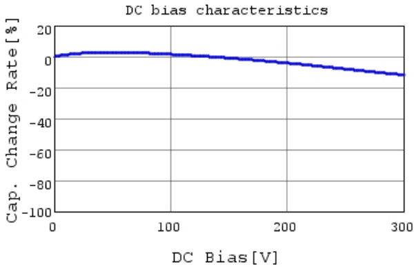
DE2F3KY103MA3BU02F C-DC bias capchange, 20.0
