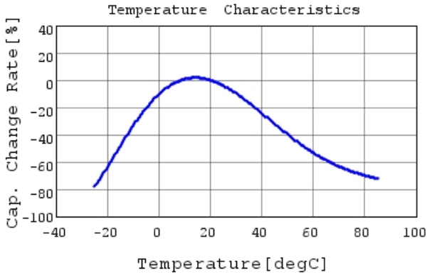
DE2F3KY103MA3BU02F C-Temp. capchange, DCOV,
