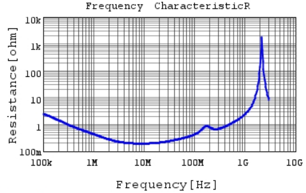
DE2F3KY103MA3BU02F R DC0V, 20degC
