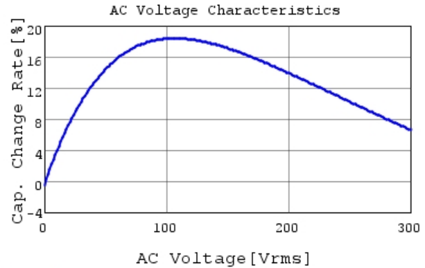
DE2F3KY103MA3BU02F C-AC Voltage capchange, I
