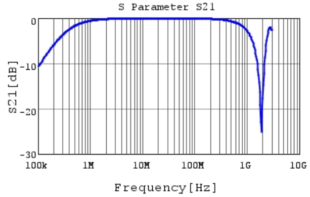
DE1E3KX472MB4BP01F S21 DC0V, 20degC
