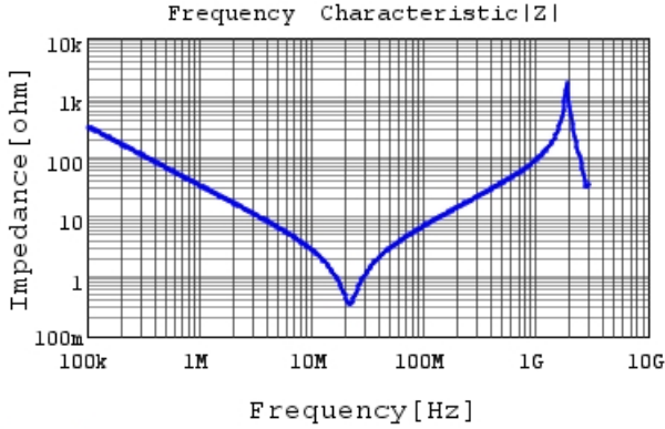
DE1E3KX472MB4BP01F |Z| DC0V, 20degC
