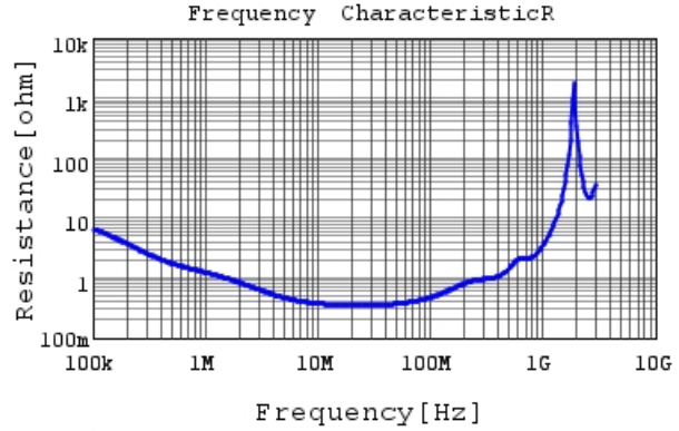
DE1E3KX472MB4BP01F R DC0V, 20degC
