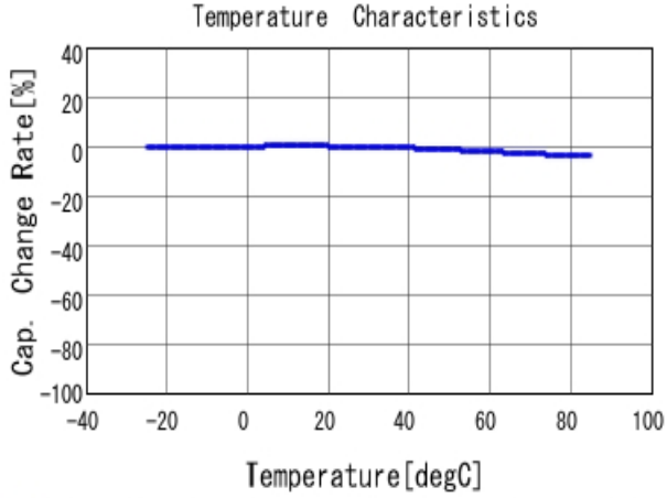
■ DE2B3KY101KB2BM01F C-Temp. capchange, DCOV, AC1Vrms
