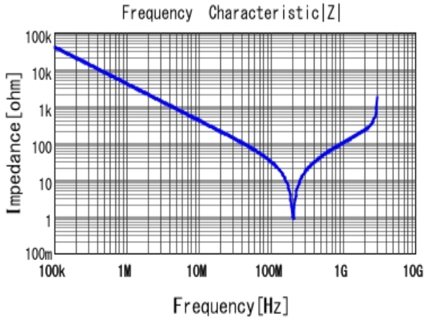
■ DE2B3KY101KB2BM01F |Z| DC0V, 20degC
