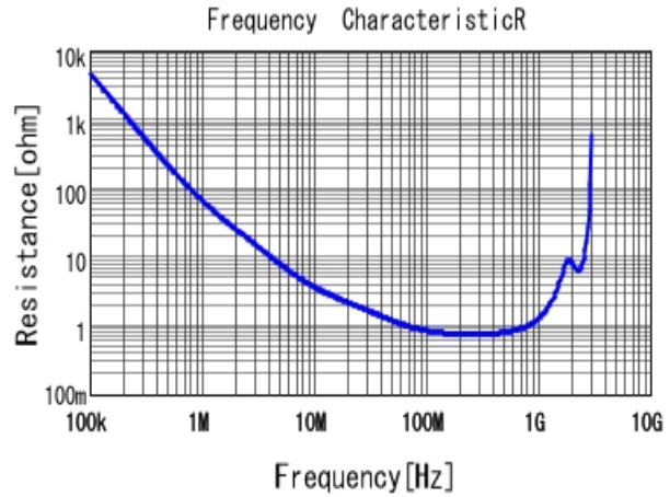
■ DE2B3KY101KB2BM01F R DC0V, 20degC
