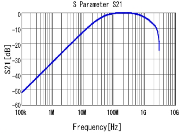
■ DE2B3KY101KB2BM01F S21 DCOV, 20degC
