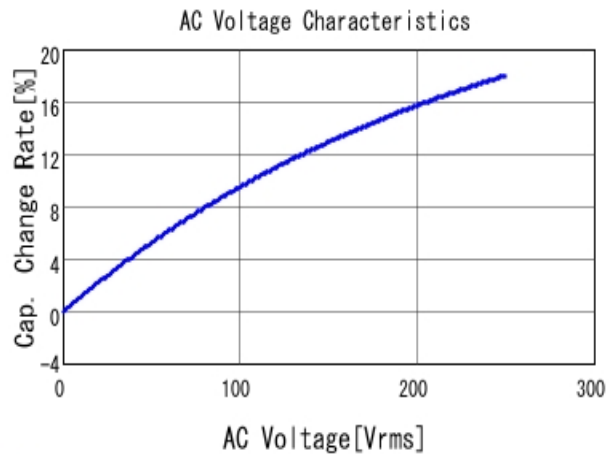
■ DE2B3KY101KB2BM01F C-AC Voltage capchange, DC0V, 20.0
