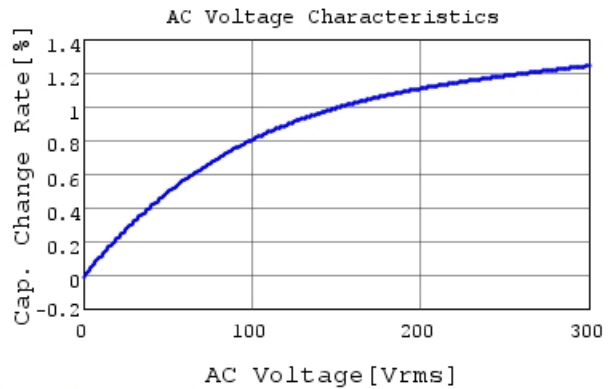
DE11XRA220KN4AP01F C-AC Voltage capchange, I
