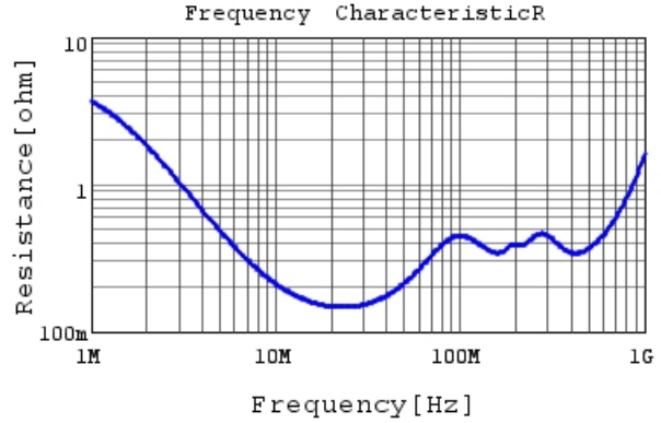
DE11XRA220KN4AP01F R DCOV, 20degC
