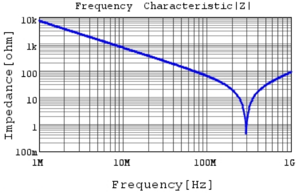
DE11XRA220KN4AP01F |Z| DCOV, 20degC
