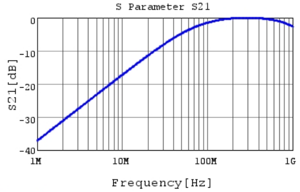
DE11XRA220KN4AP01F S21 DCOV, 20degC
