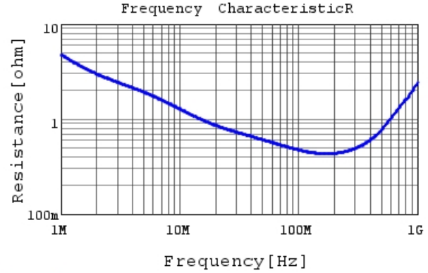
DE1E3RA102MN4AN01F R DCOV, 20degC
