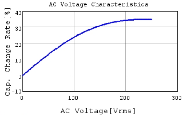
DE1E3RA102MN4AN01F C-AC Voltage capchange, I
