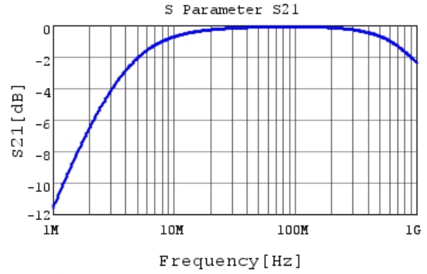
DE1B3RA471KA4BQ01F S21 DCOV, 20degC
