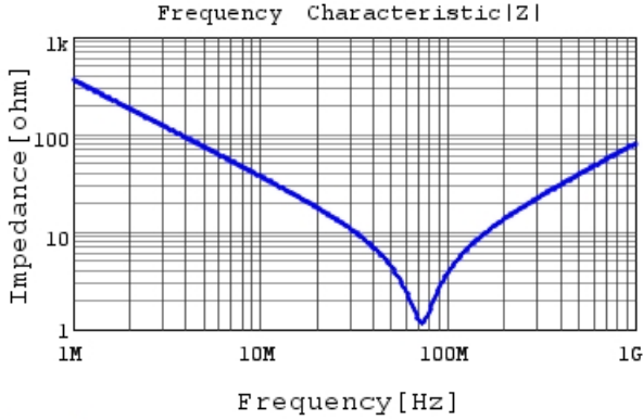
DE1B3RA471KA4BQ01F |Z| DC0V, 20degC
