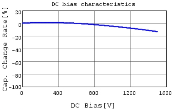
DE1B3RA471KA4BQ01F C-DC bias capchange, 20.0
