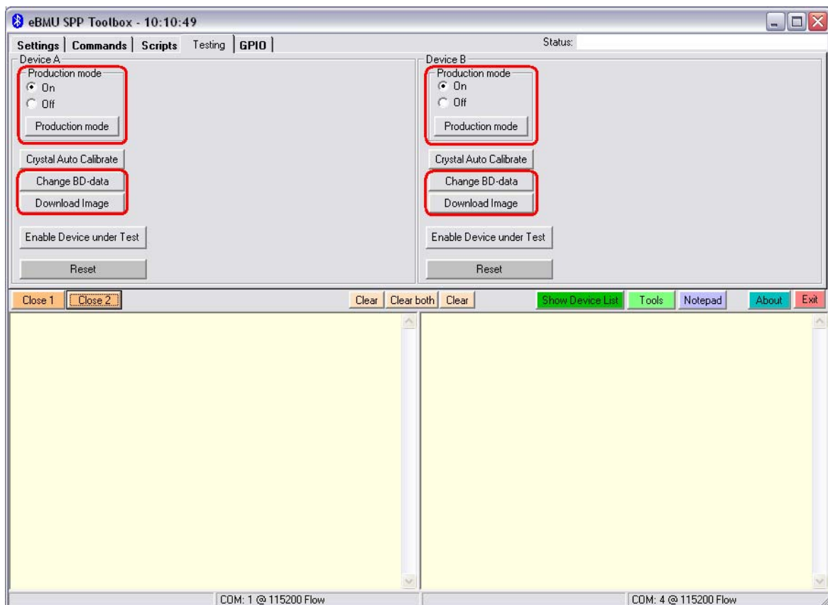
Figure 6 : Testing tab
