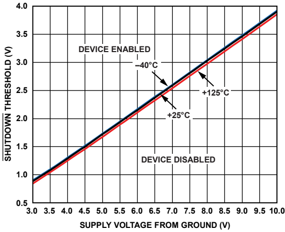
Figure 43. SHUTDOWN Threshold vs. Supply Voltage from Ground for Various Temperatures
