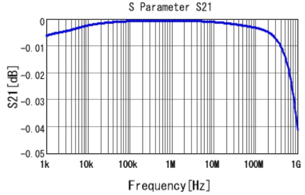
■ ECASD40G107M016K00 S21 DCOV, 25degC
