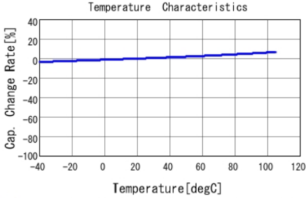
■ ECASD40G107M016K00 C-Temp. capchange, DCOV, AC1Vrms
