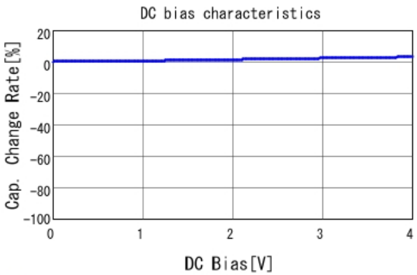
■ ECASD40G107M016K00 C-DC bias capchange, 25.0degC, AC1
