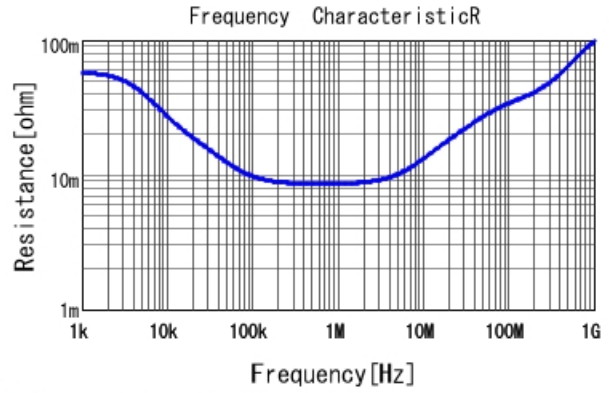
■ ECASD40G107M016K00 R DCOV, 25degC
