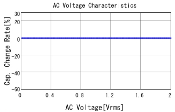
■ ECASD40G107M016K00 C-AC Voltage capchange, DCOV, 25.0
