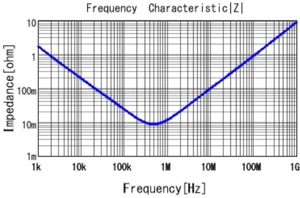
■ ECASD40G107M016K00 |Z| DCOV, 25degC
