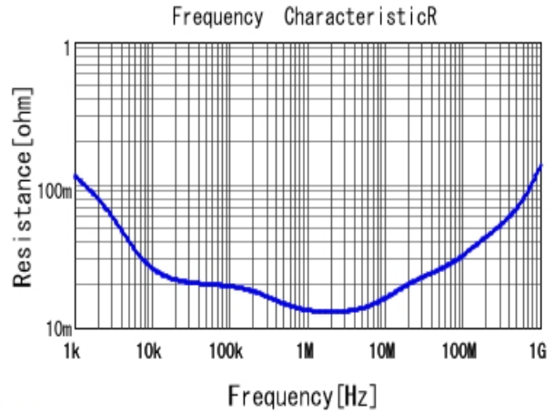
■ ECASD41E106M040KA0 R DCOV, 25degC
