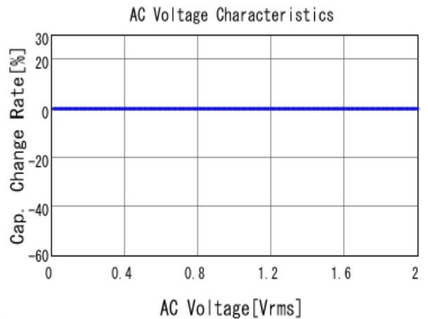
■ ECASD41E106M040KA0 C-AC Voltage capchange, DCOV, 25.0
