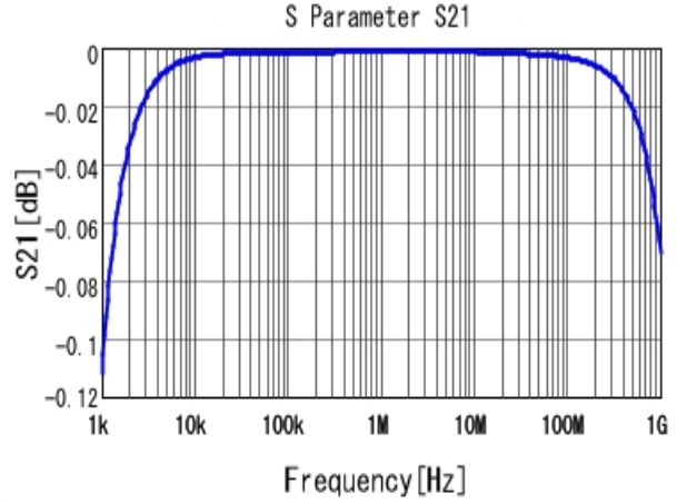
■ ECASD41E106M040KA0 S21 DCOV, 25degC
