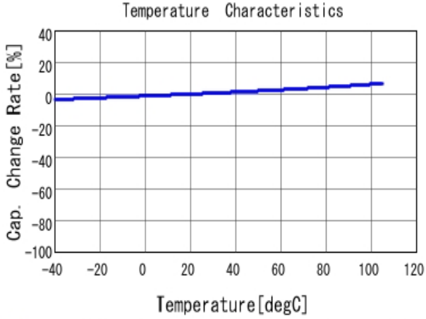
■ ECASD41E106M040KA0 C-Temp. capchange, DCOV, AC1Vrms
