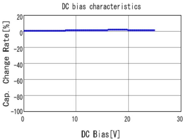
■ ECASD41E106M040KA0 C-DC bias capchange, 25.0degC, AC1
