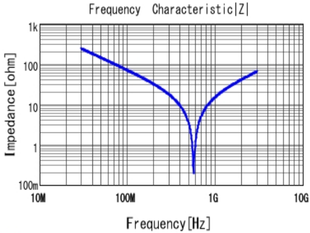
■ RCE5C2A220J0DBH03A |Z| DC0V, 25degC
