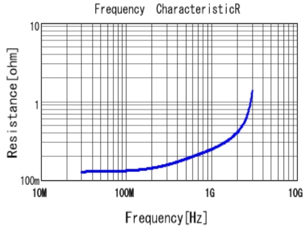
■ RCE5C2A220J0DBH03A R DC0V, 25degC
