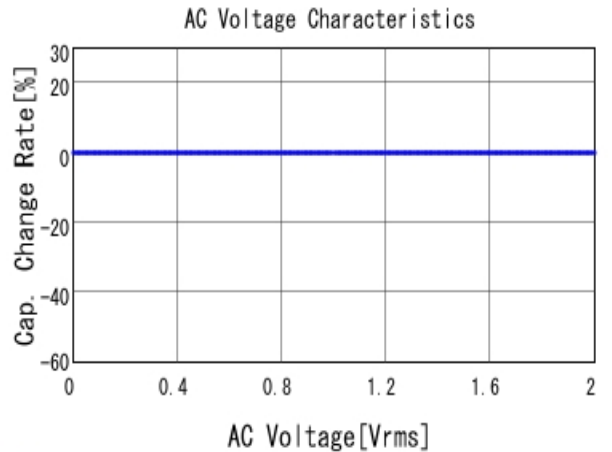
■ RCE5C2A220J0DBH03A C-AC Voltage capchange, DC0V, 25.0
