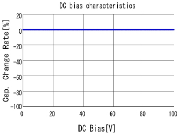
■ RCE5C2A220J0DBH03A C-DC bias capchange, 25.0degC, AC1
