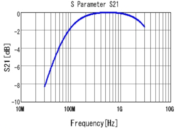
■ RCE5C2A220J0DBH03A S21 DCOV, 25degC
