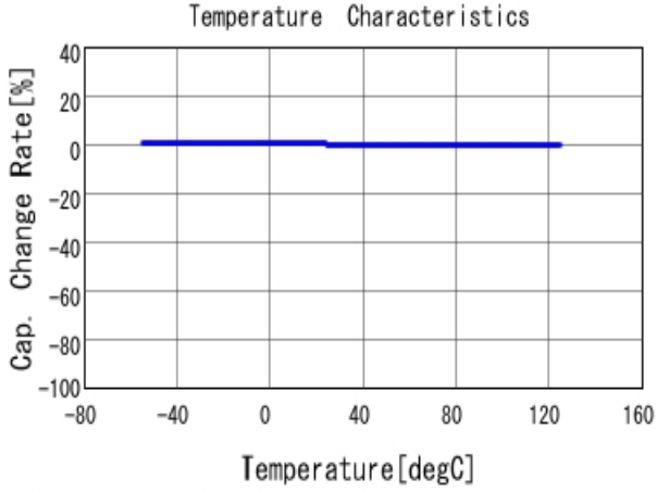
■ RCE5C2A220J0DBH03A C-Temp. capchange, DCOV, AC1Vrms
