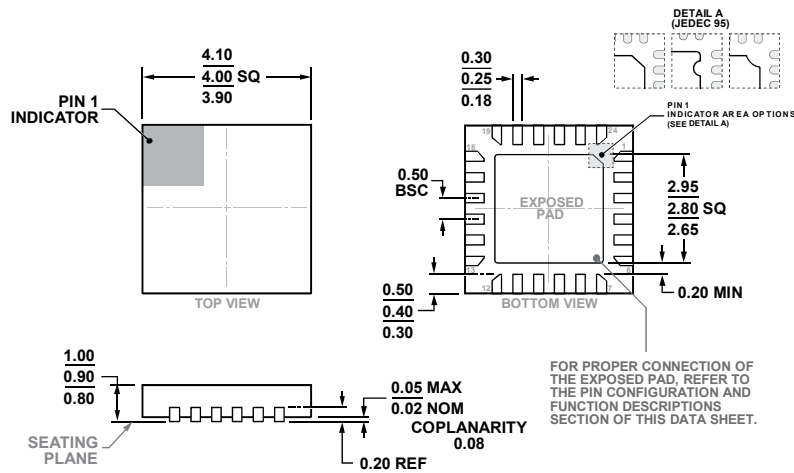
Figure 55. 24-Lead Lead Frame Chip Scale Package [LFCSP] 4 mm × 4 mm Body and 0.90 mm Package Height (HCP-24-2) Dimensions shown in millimeters
