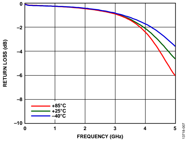
Figure 7. RF1 Return Loss vs. Frequency over Temperature, V_{DD} = 3 V , V_{CTL} = 0 V
