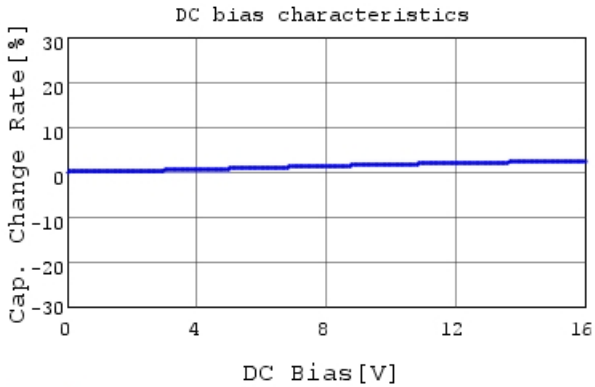
ECASD41C686M040KA0 C-DC bias capchange, 25.0
