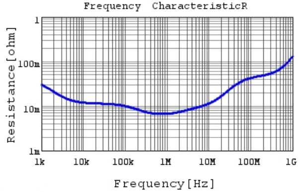
ECASD41C686M040KA0 R DCOV, 25degC
