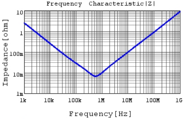
ECASD41C686M040KA0 |Z| DCOV, 25degC
