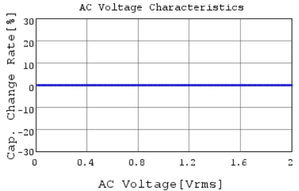
ECASD41C686M040KA0 C-AC Voltage capchange, 1
