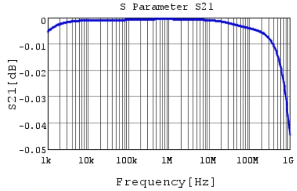
ECASD41C686M040KA0 S21 DCOV, 25degC
