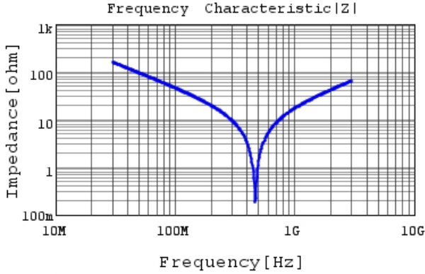
RCE5C2A330J0DBH03A |Z| DCOV, 25degC
