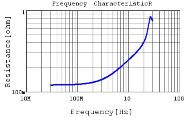
RCE5C2A330J0DBH03A R DCOV, 25degC
