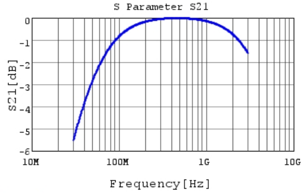
RCE5C2A330J0DBH03A S21 DC0V, 25degC
