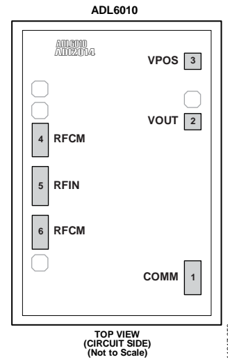
Figure 3. 6-Pad Bare Die Pin Configuration
