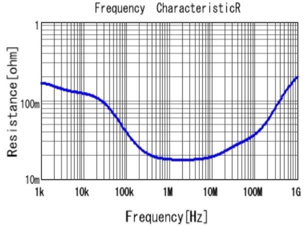
■ ECASD40J106M055K00 R DCOV, 25degC
