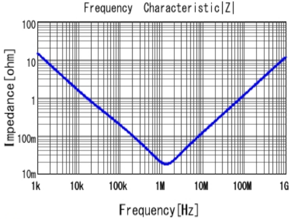
■ ECASD40J106M055K00 |Z| DCOV, 25degC
