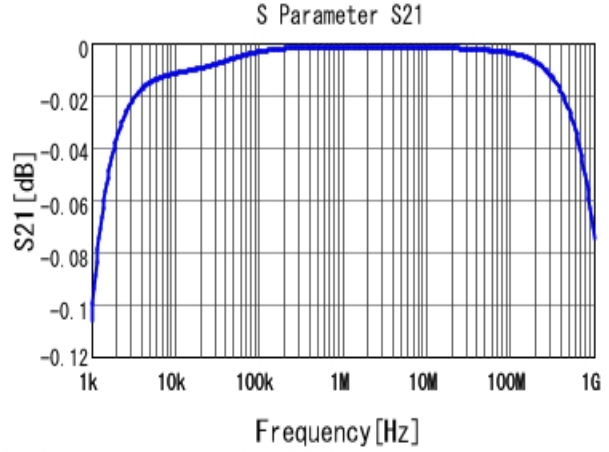
■ ECASD40J106M055K00 S21 DCOV, 25degC
