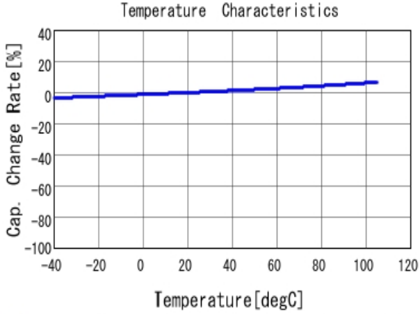
■ ECASD40J106M055K00 C-Temp. capchange, DCOV, AC1Vrms
