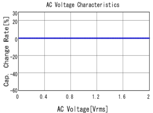
■ ECASD40J106M055K00 C-AC Voltage capchange, DCOV, 25.0
