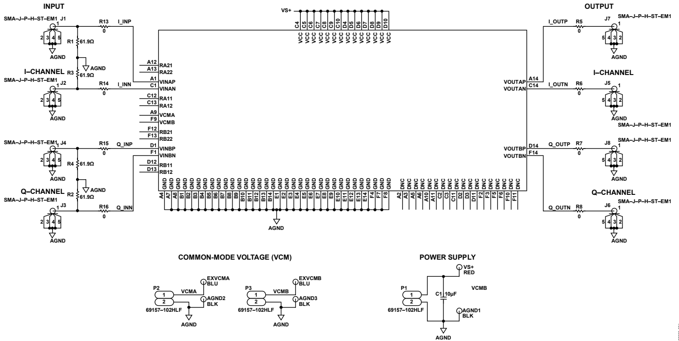
Figure 7. EVAL-ADAQ8088EBZ Schematic
