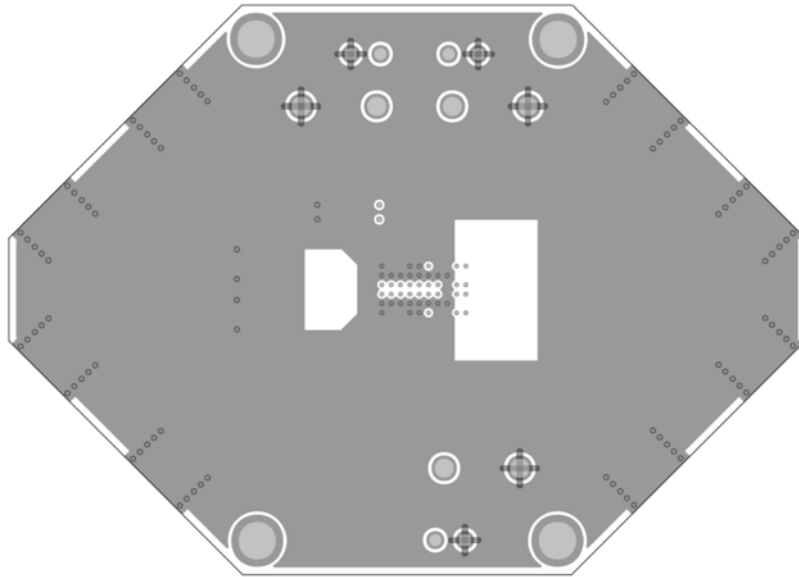
Figure 10. EVAL-ADAQ8088EBZ GND Plane
