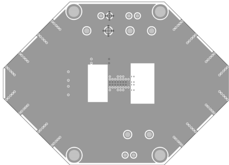
Figure 11. EVAL-ADAQ8088EBZ Power Plane
