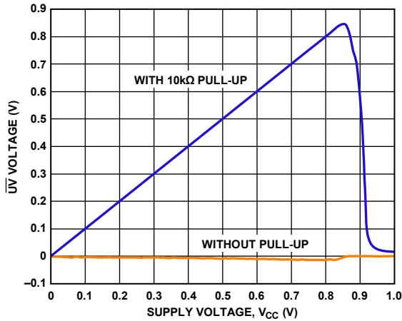
Figure 10. \overline{UV} Output Voltage vs. V_{CC}
