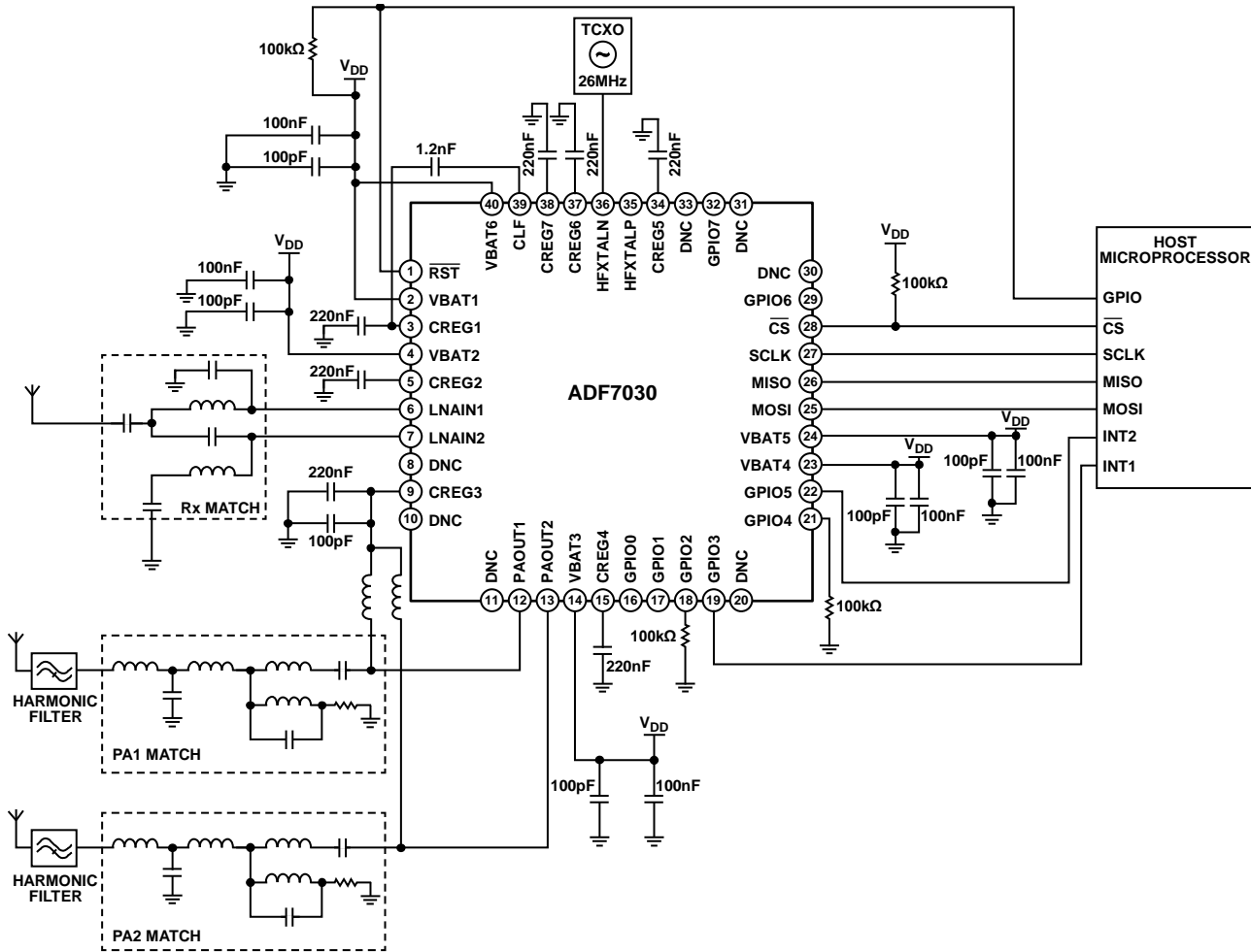
Figure 39. Application Circuit with Both PAs and LNA Matched, Without External PA or Tx/Rx Switch
