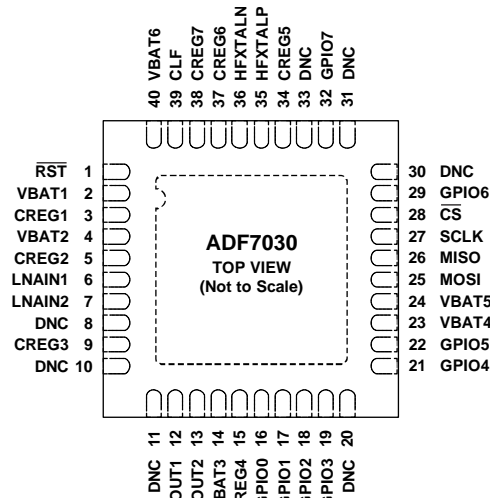
Figure 4. Pin Configuration
