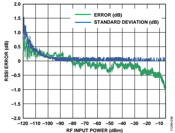
Figure 21. RSSI Error vs. RF Input Power with One-Point Calibration at -70\text{ dBm} , V_{DD} = 2.2\text{ V} , T_A = 25^\circ\text{C} (Error is Based on the Mean of 20 RSSI Measurements)
