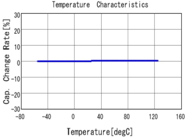
■ GCQ1555C1H8R8CB01 C-Temp. capchange, DCOV, AC1Vrms
