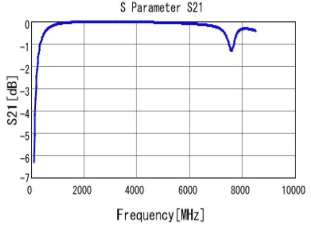
■ GCQ1555C1H8R8CB01 S21 DCOV, 25degC
