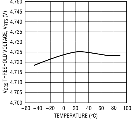
V CC5 Threshold Voltage vs Temperature (LTC1326)
