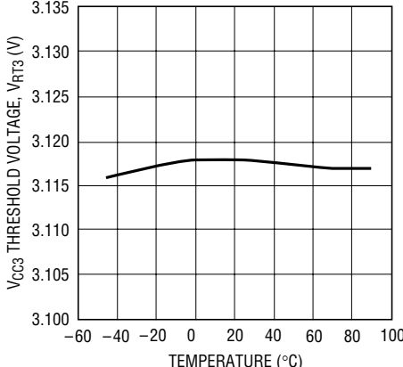
V CC3 Threshold Voltage vs Temperature
