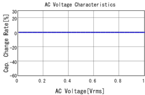
■ ECASD60E477M4R5K00 C-AC Voltage capchange, DC0V, 25.0
