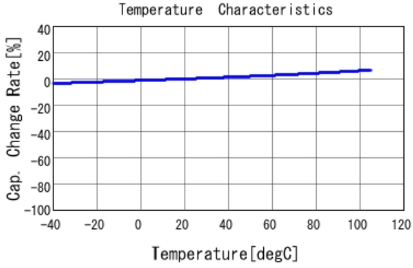
■ ECASD60E477M4R5K00 C-Temp. capchange, DCOV, AC1Vrms
