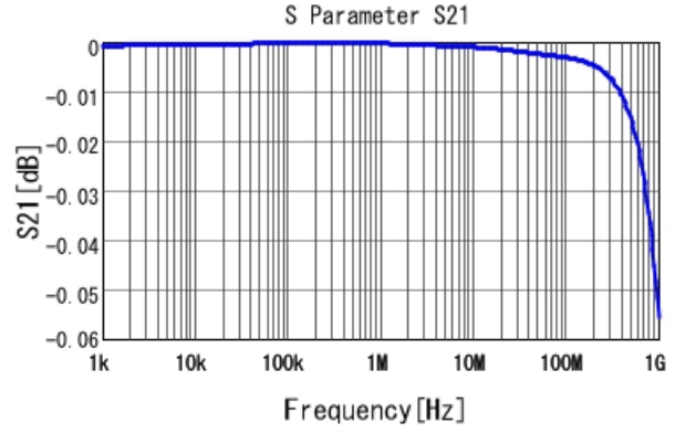
■ ECASD60E477M4R5K00 S21 DCOV, 25degC
