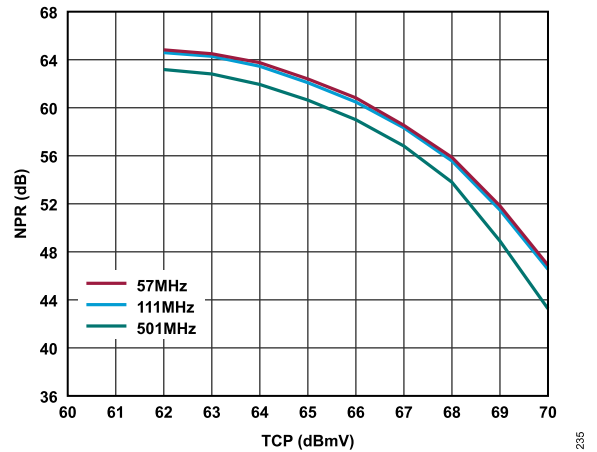
Figure 37. NPR vs. TCP Over Frequency, 0 dB Tilt, V_{DD} = 8.0 V
