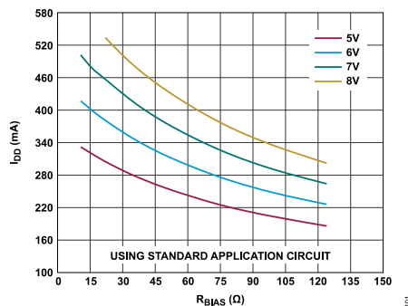
Figure 42. I_{DD} vs. R_{BIAS} over V_{DD}
