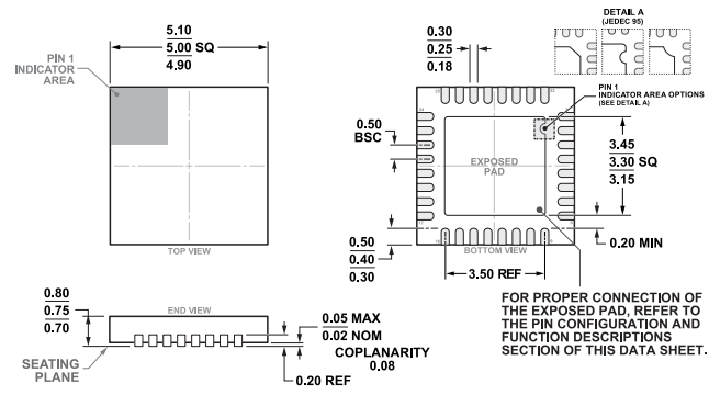
Figure 43. 32-Lead Lead Frame Chip Scale Package [LFCSP] 5 mm × 5 mm Body and 0.75 mm Package Height (CP-32-13) Dimensions shown in millimeters
