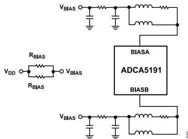
Figure 41. Suggested BIASA and BIASB Application Circuit
