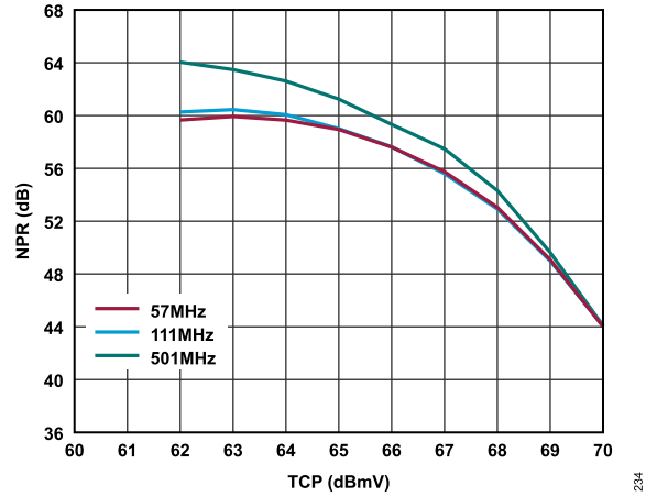
Figure 36. NPR vs. TCP Over Frequency, 10 dB Tilt, V_{DD} = 8.0 V
