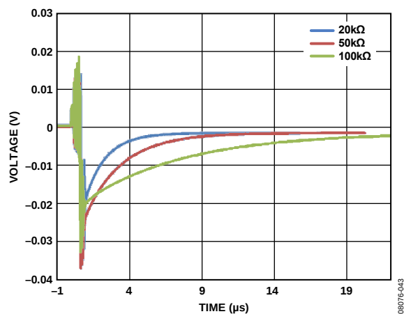
Figure 31. Maximum Glitch Energy
