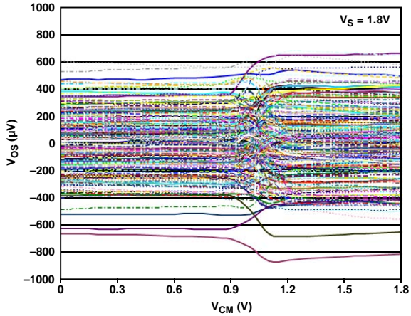
Figure 26. Input Offset Voltage vs. Input Common-Mode Voltage
