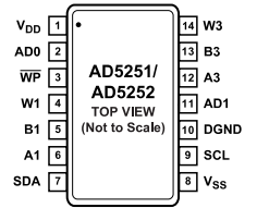
Figure 2. Pin Configuration
