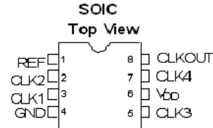
Figure 2. Pin Configuration – CY23S05
