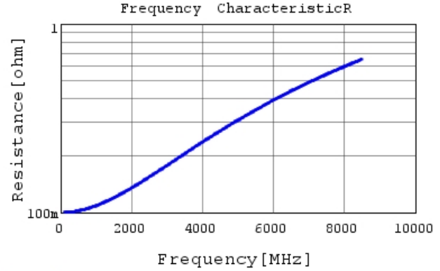
GJM0335C1E7R9CB01 R DC0V, 25degC
