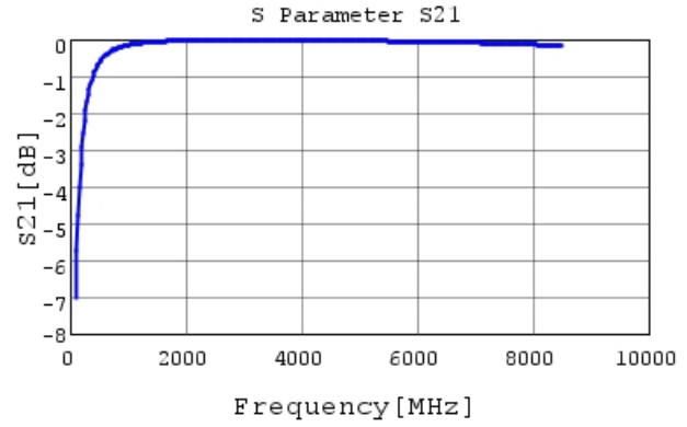
GJM0335C1E7R9CB01 S21 DCOV, 25degC
