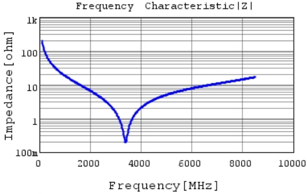
GJM0335C1E7R9CB01 |Z| DC0V, 25degC
