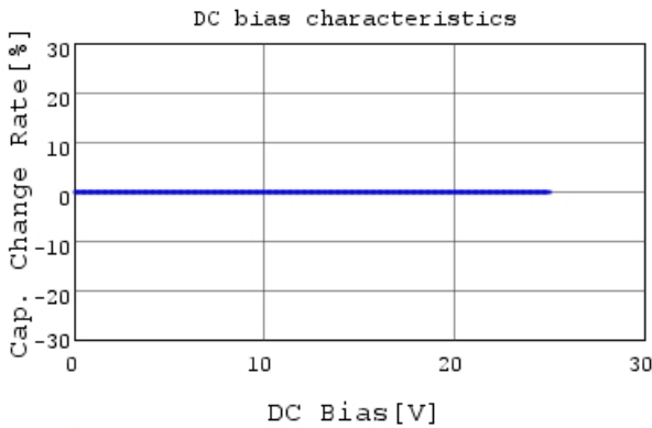
GJM0335C1E7R9CB01 C-DC bias capchange, 25.0c
