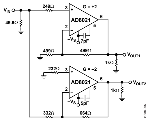
Figure 65. Differential Amplifier
