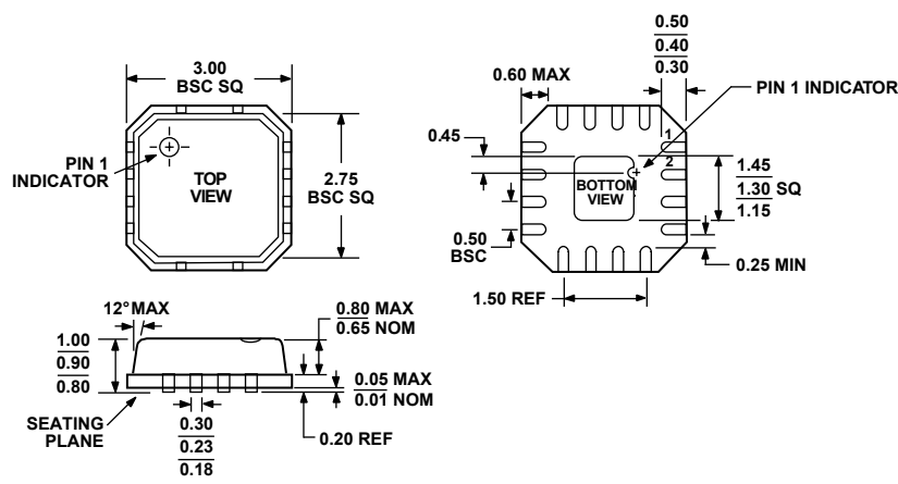
Figure 32. 16-Lead Leadframe Chip Scale Package [LFCSP] (CP-16) Dimensions shown in millimeters
