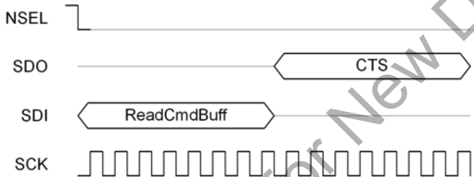
Figure 4. SPI Read Command—Check CTS Value
