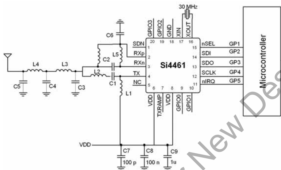
Figure 1. Si4461 Direct-Tie Application Example
