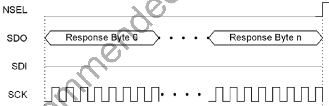
Figure 5. SPI Read Command—Clock Out Read Data
