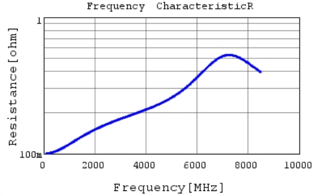
GCQ1555C1H5R3DB01 R DC0V, 25degC
