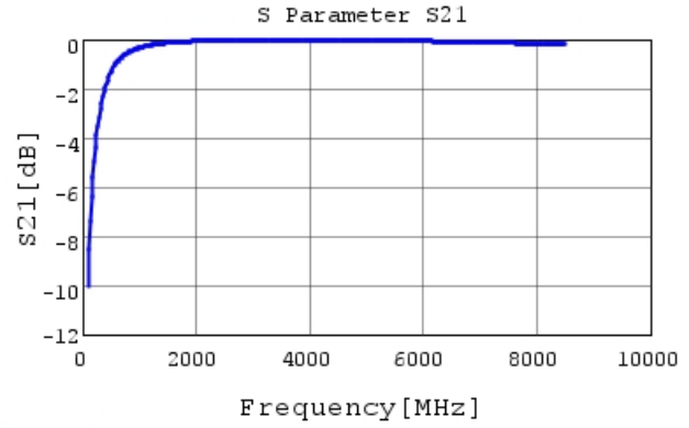
GCQ1555C1H5R3DB01 S21 DCOV, 25degC
